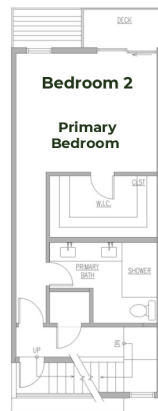
FOURTH FLOOR
