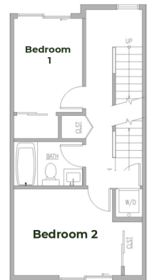
THIRD FLOOR
