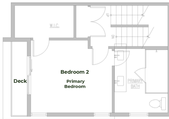
THIRD FLOOR
