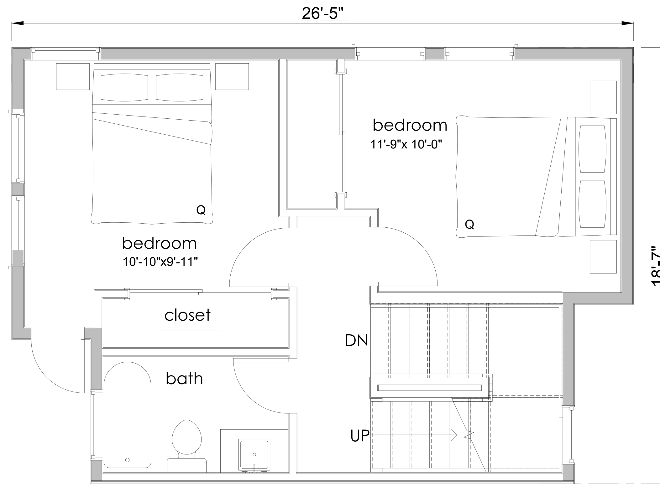
SECOND FLOOR
