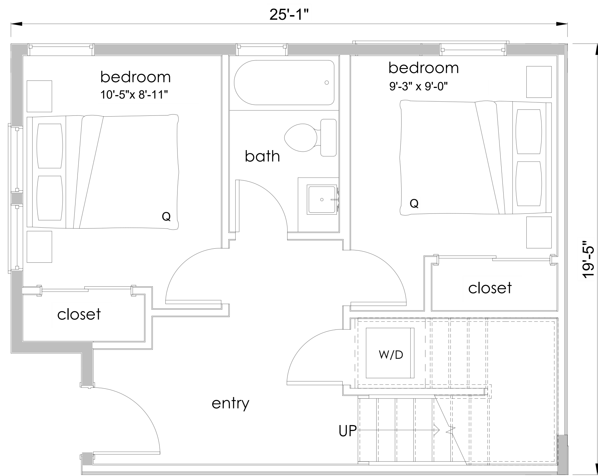
FIRST FLOOR
