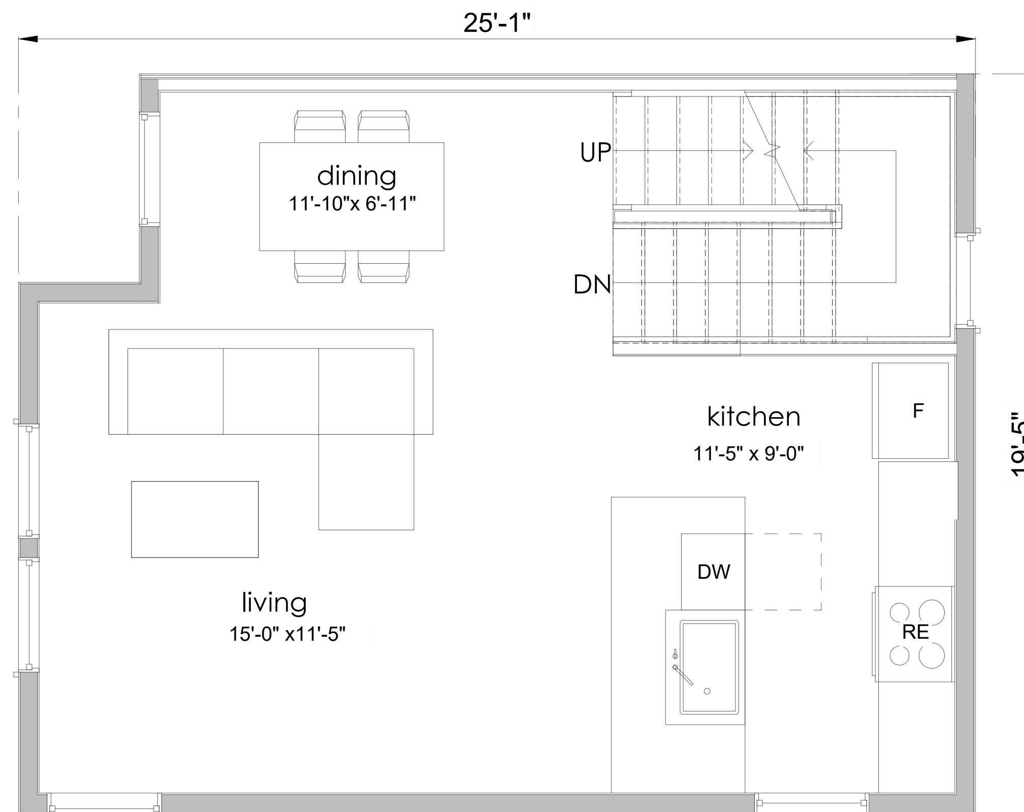
SECOND FLOOR
