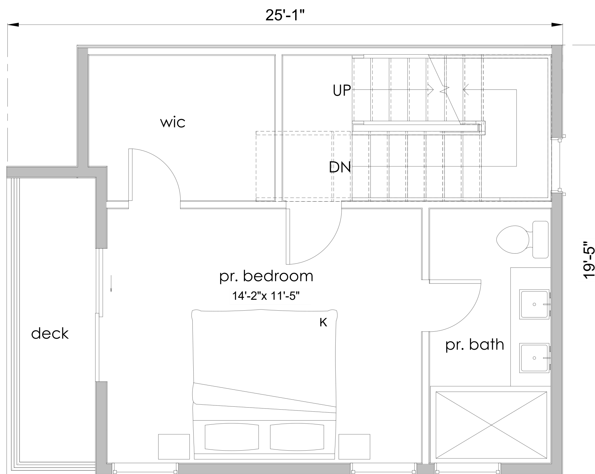
THIRD FLOOR
