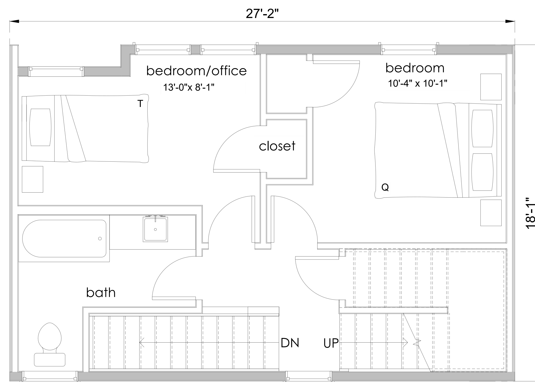
SECOND FLOOR
