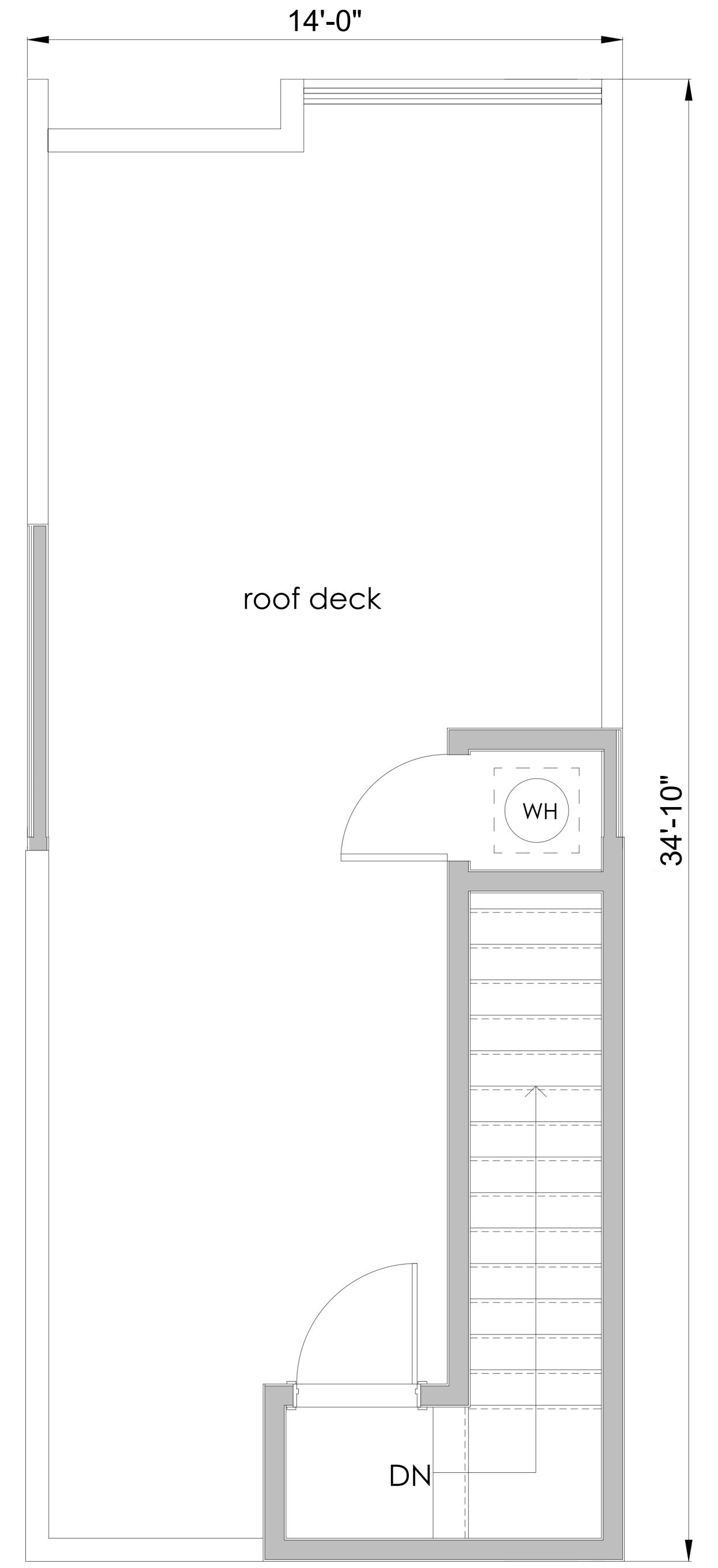
ROOF DECK
