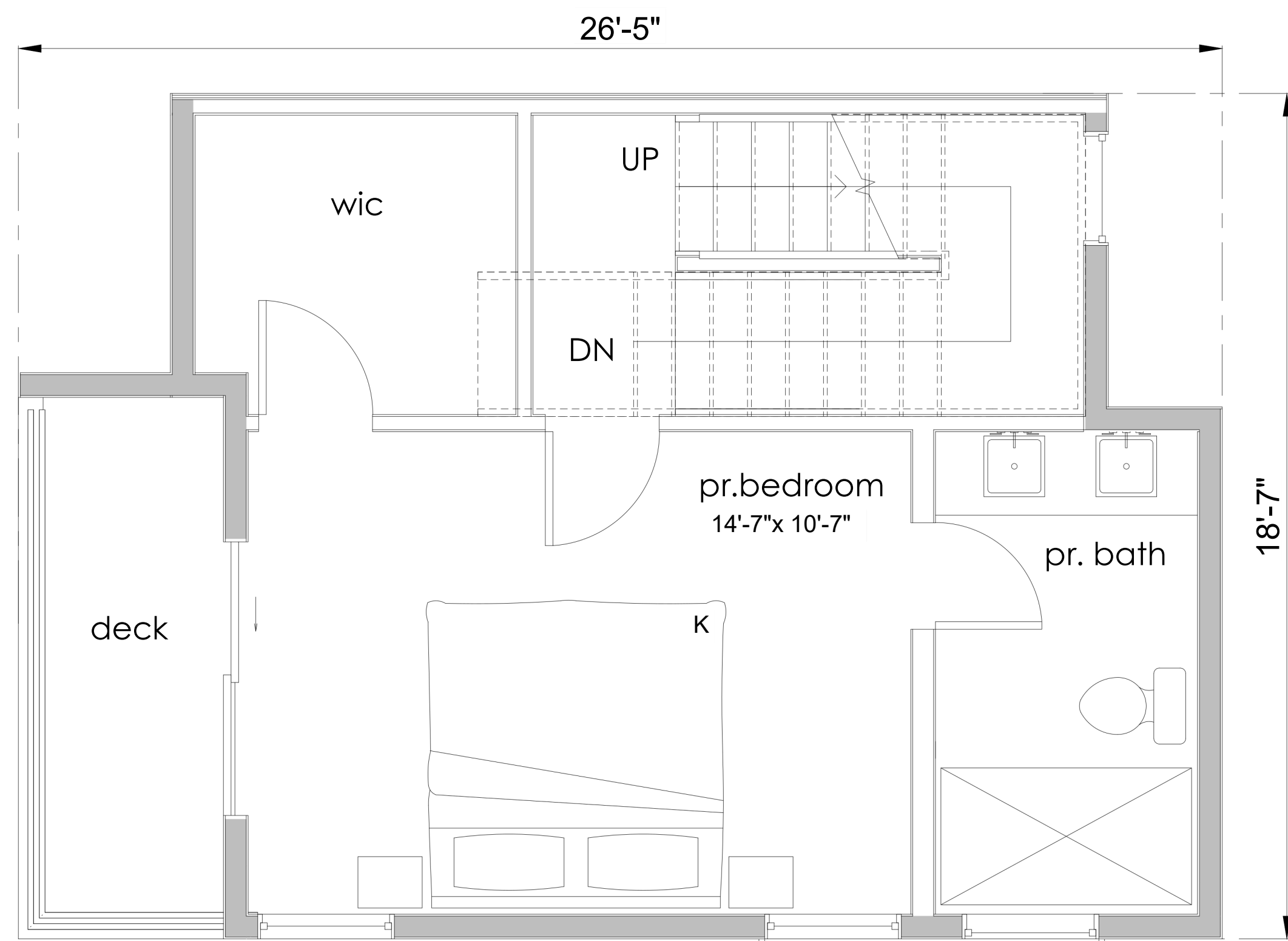
THIRD FLOOR
