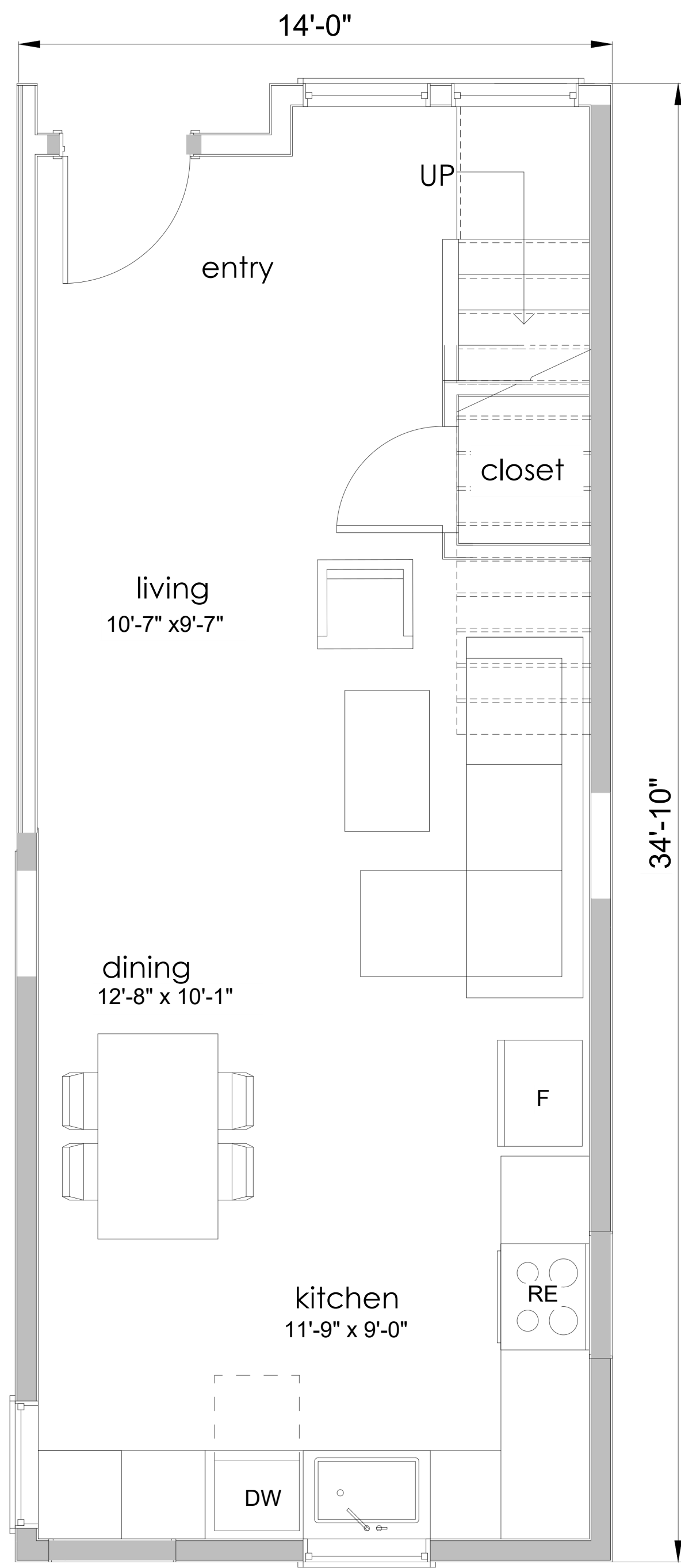
FIRST FLOOR
