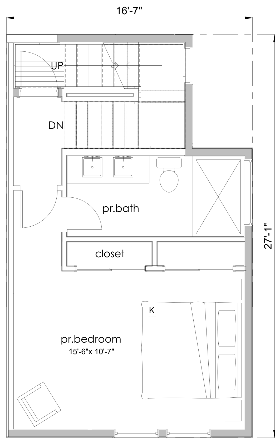
FORTH FLOOR
