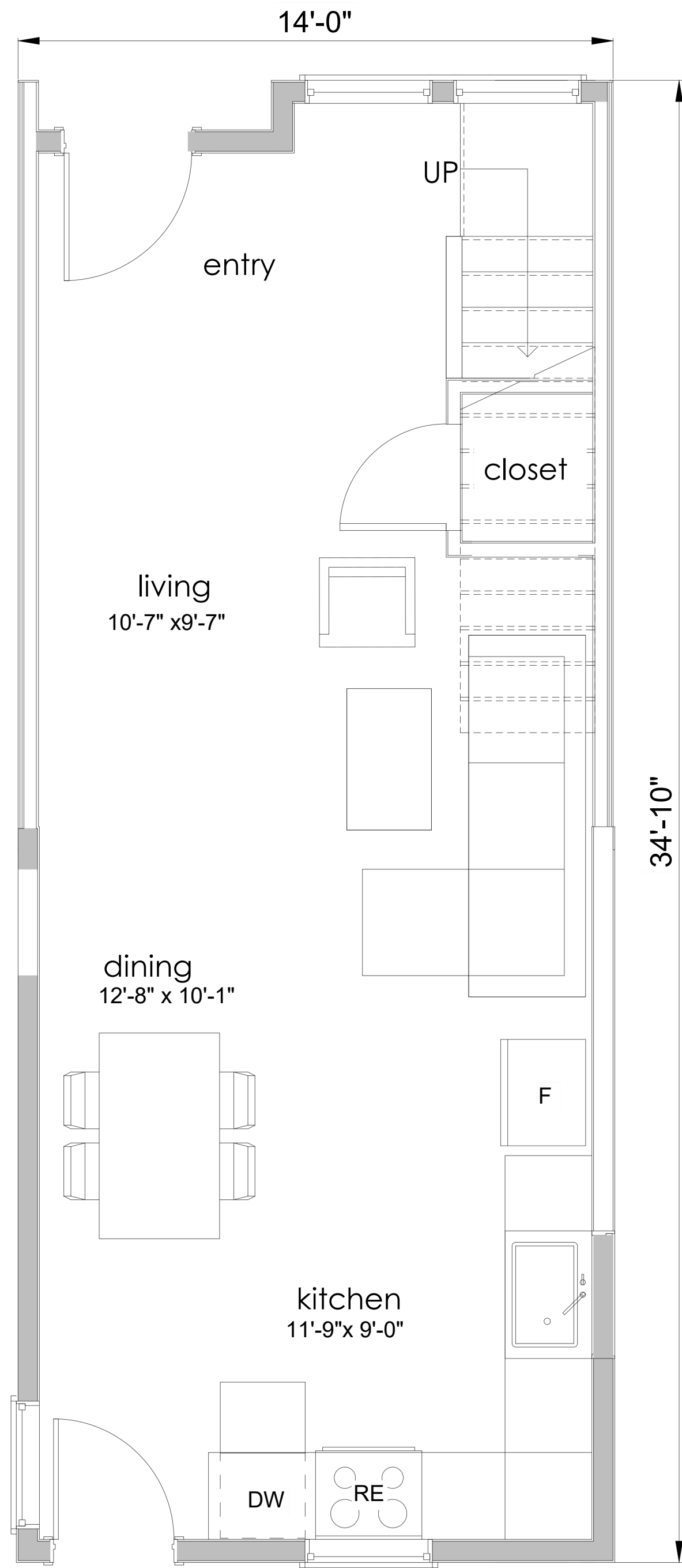
FIRST FLOOR
