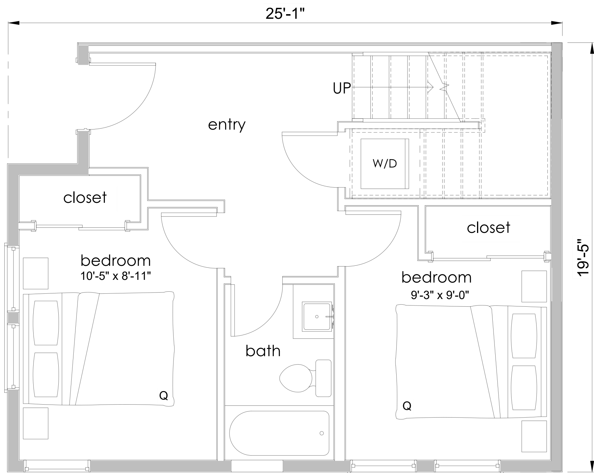
FIRST FLOOR
