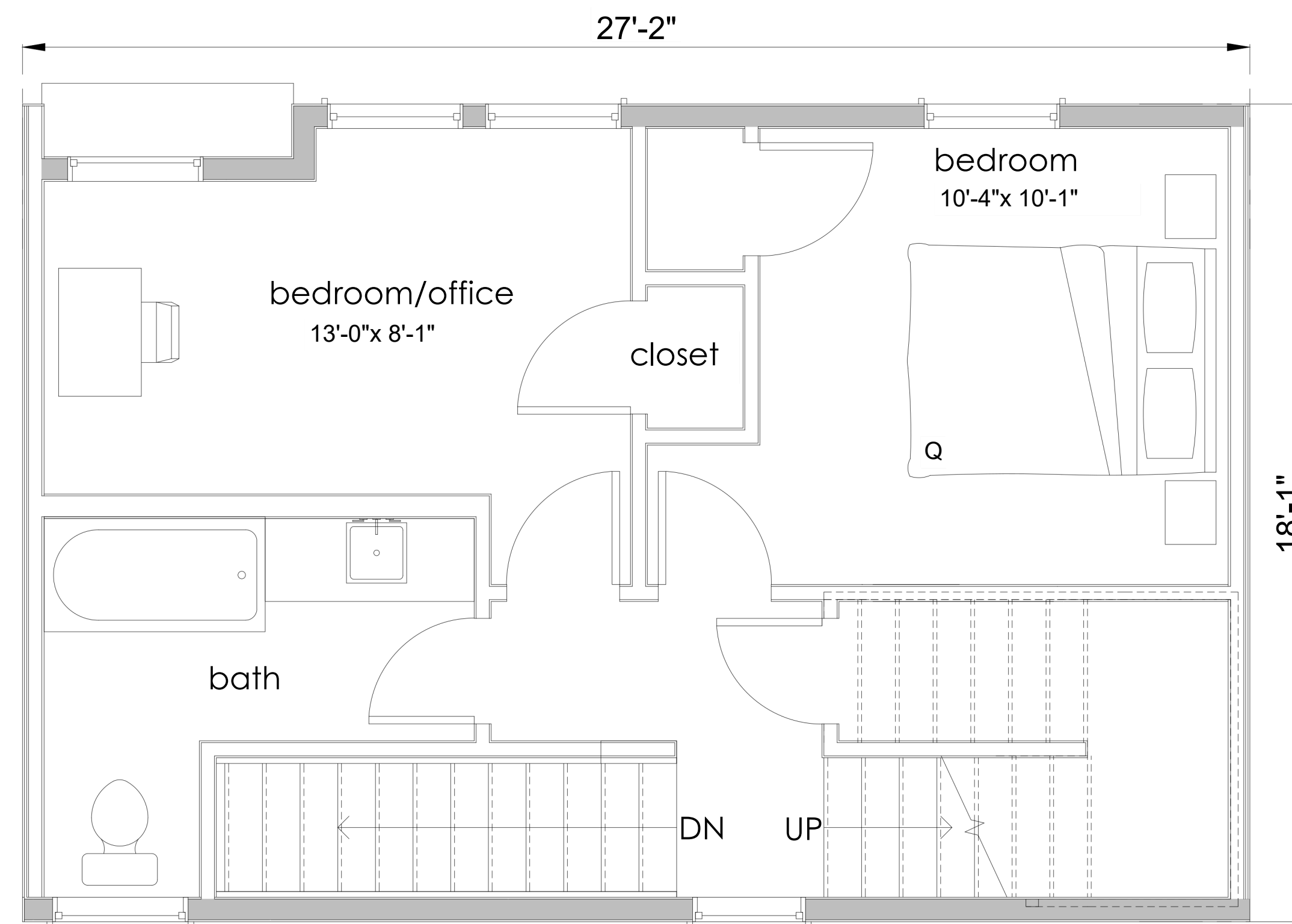
SECOND FLOOR
