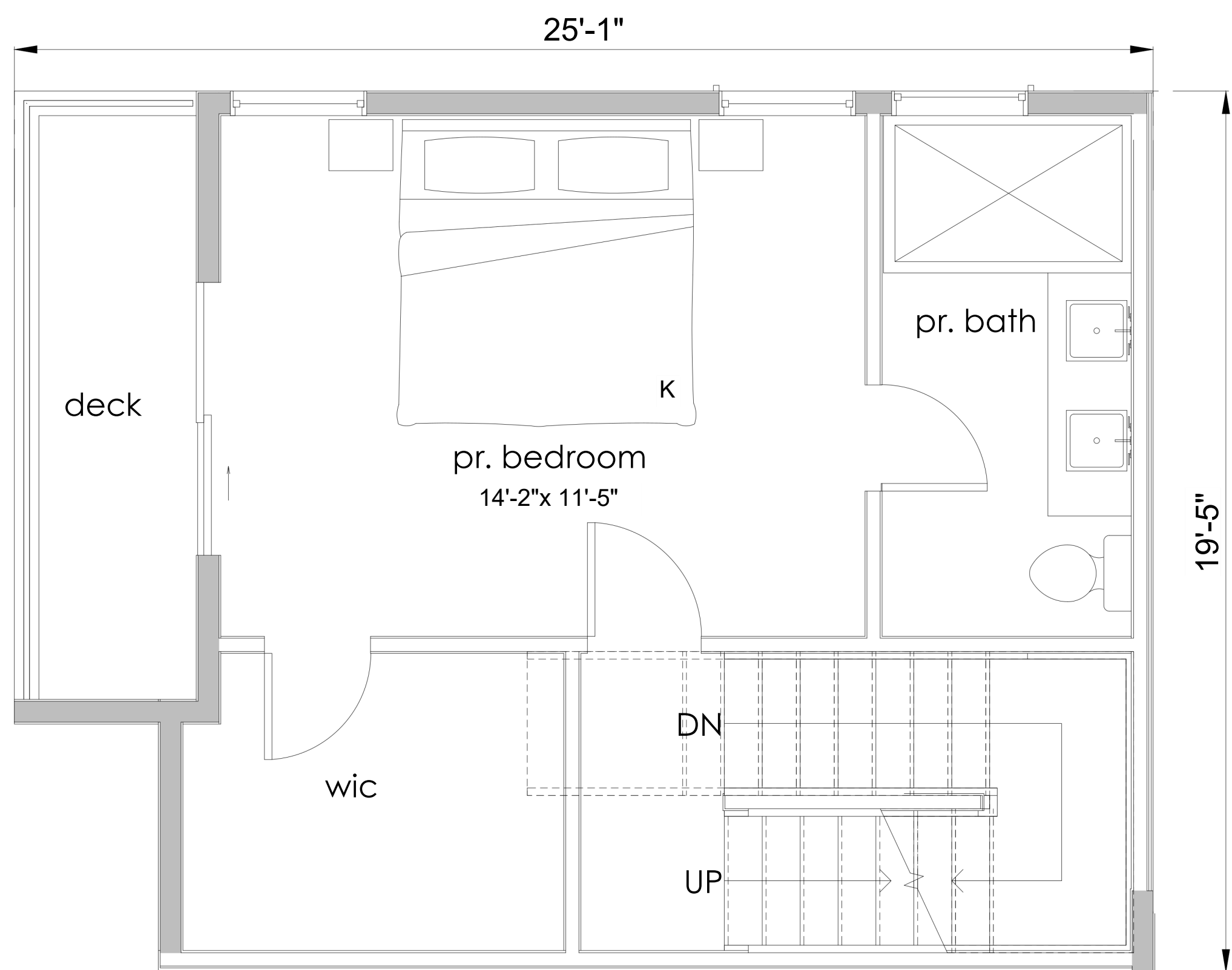
FIRST FLOOR
