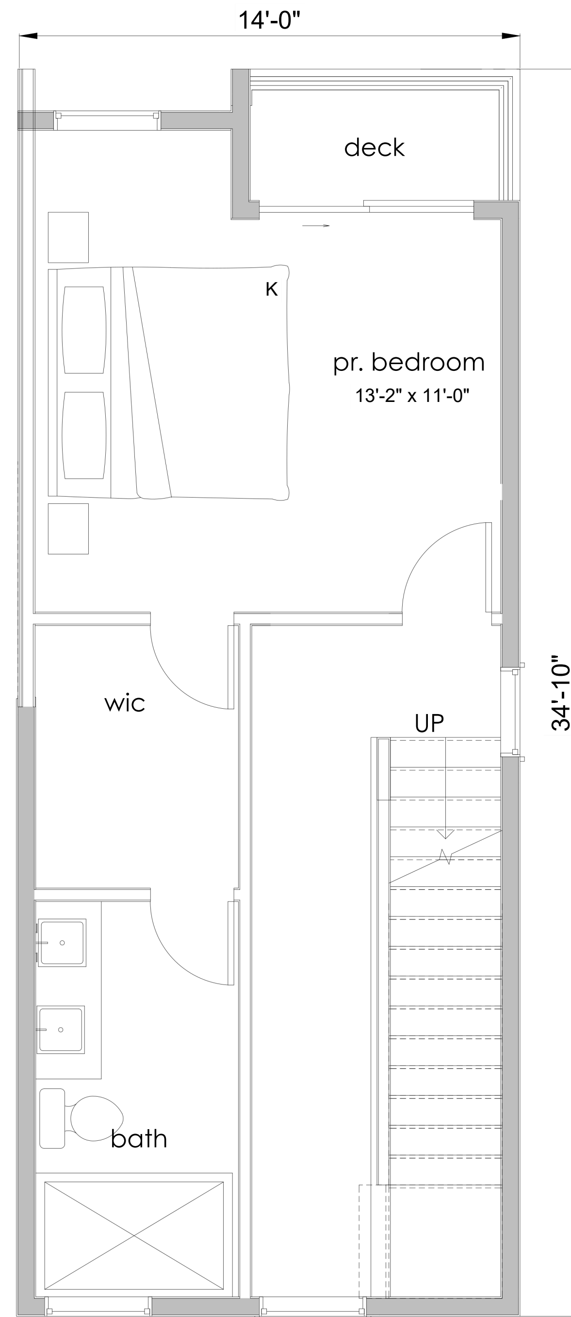
THIRD FLOOR
