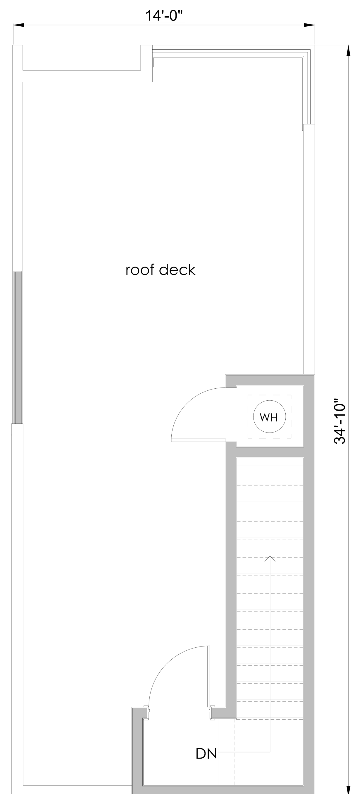
ROOF DECK
