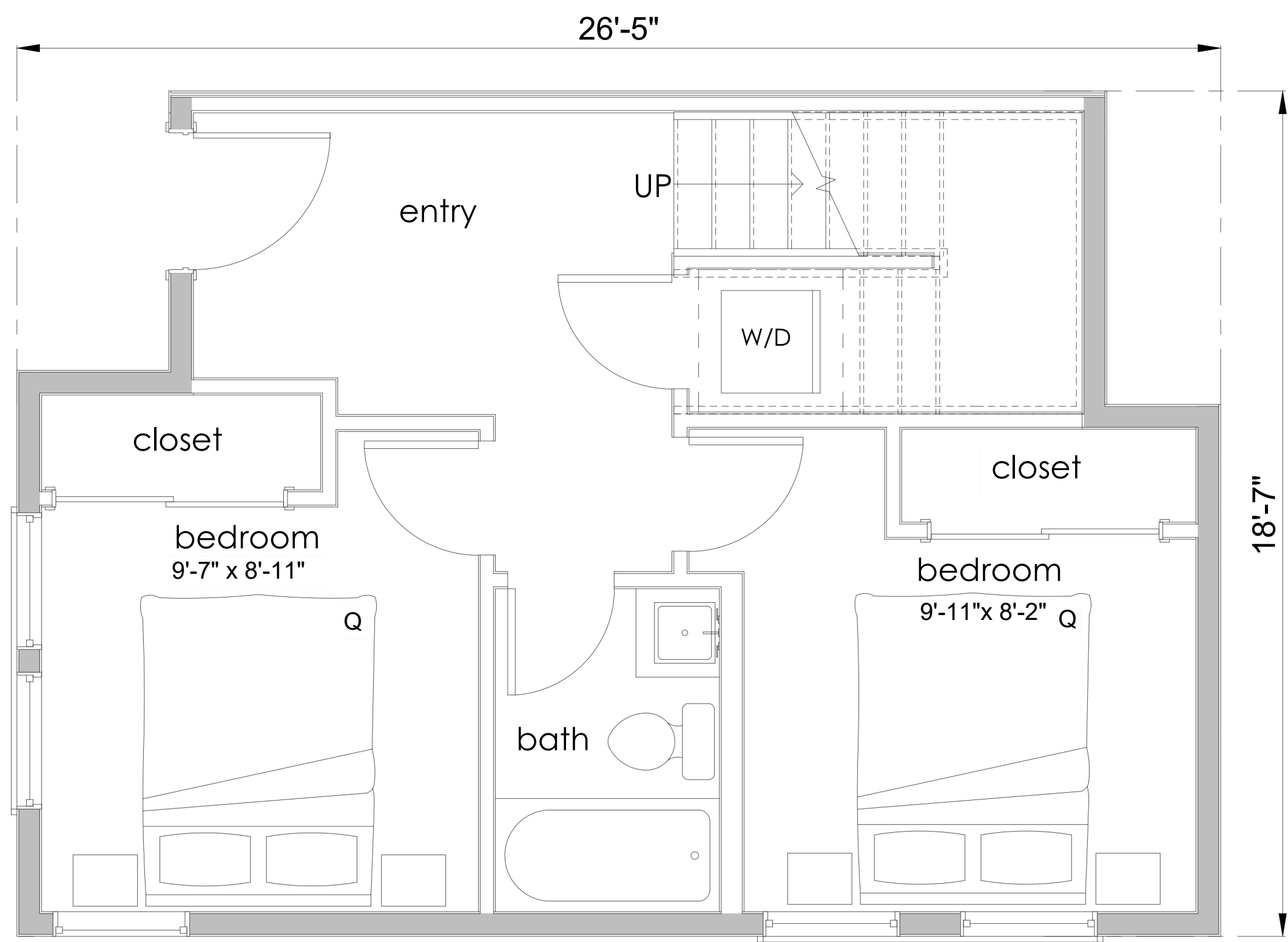
FIRST FLOOR
