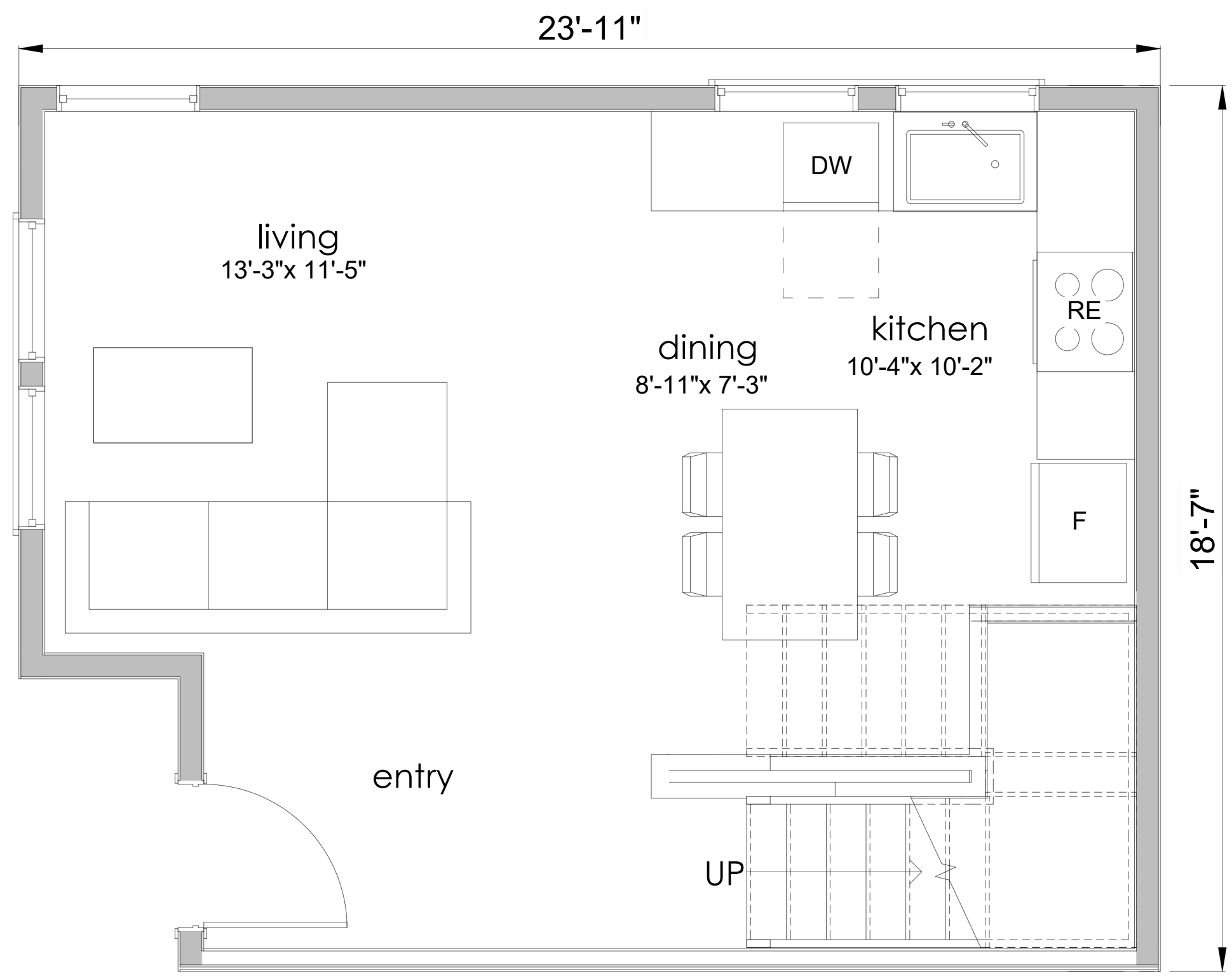
FIRST FLOOR
