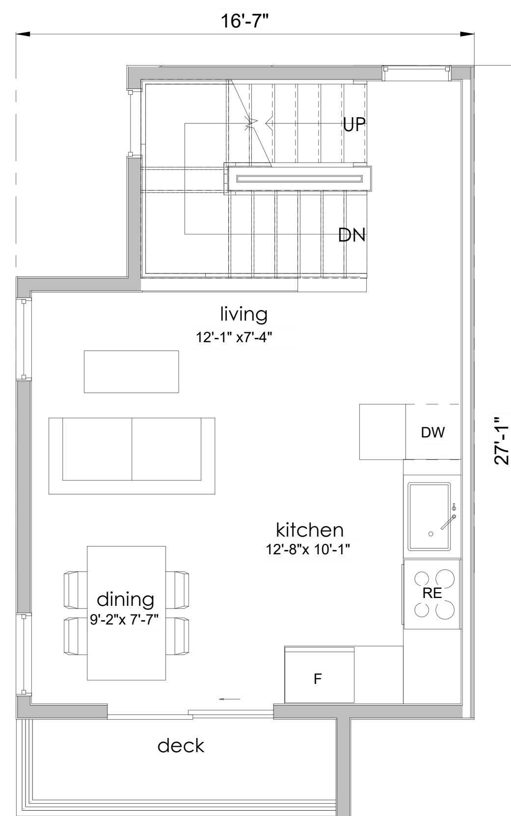
SECOND FLOOR
