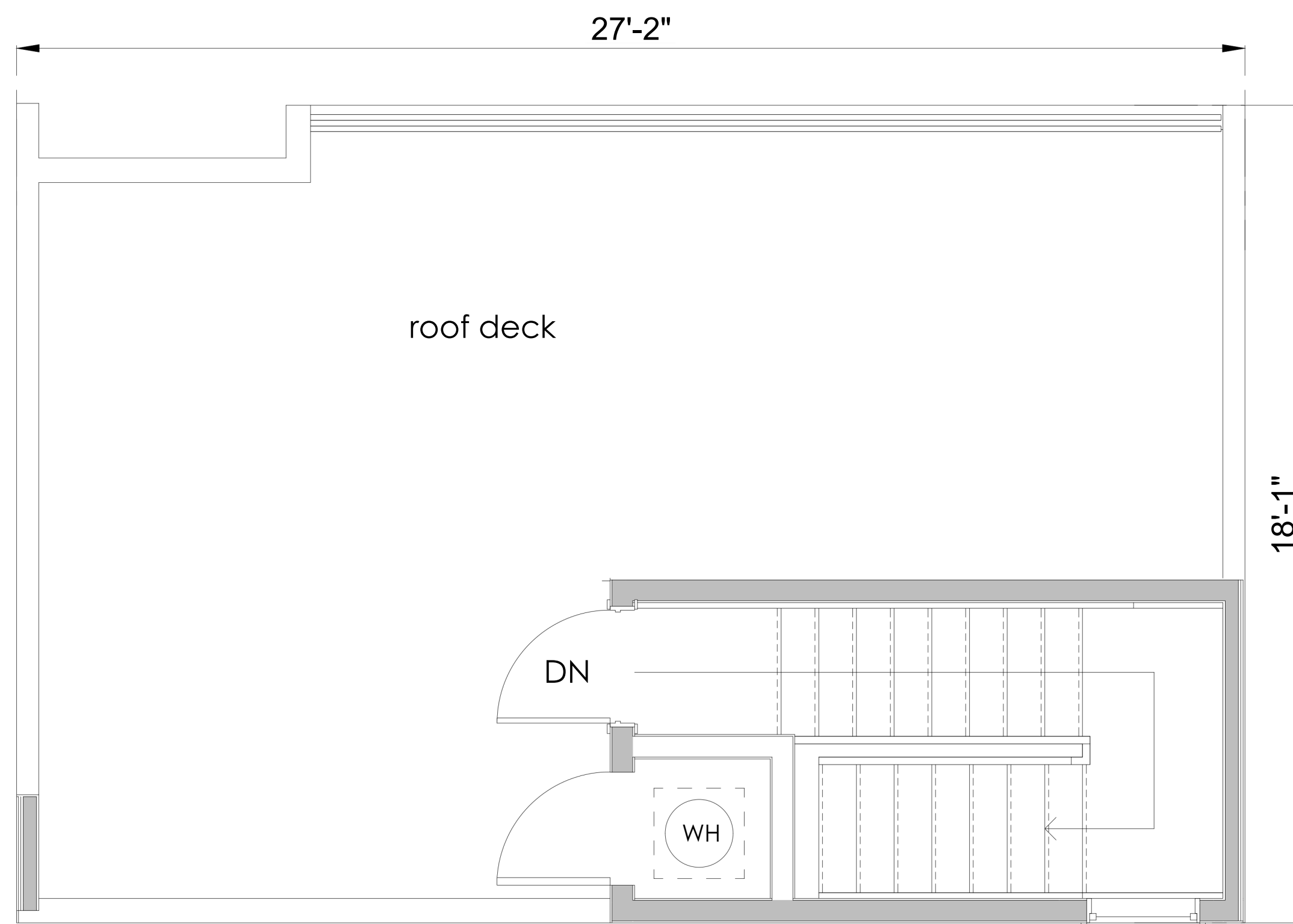
ROOF DECK
