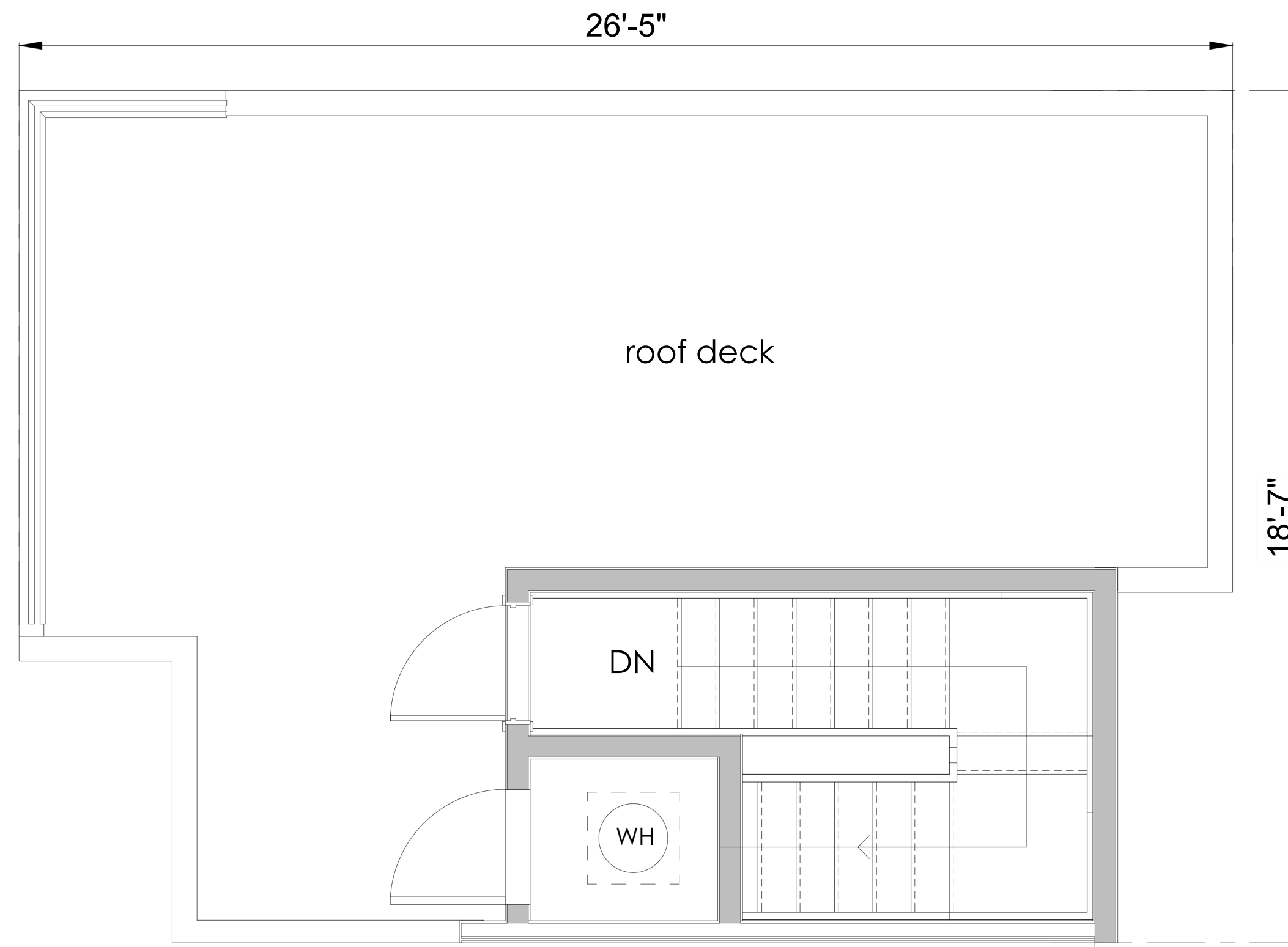
ROOF DECK
