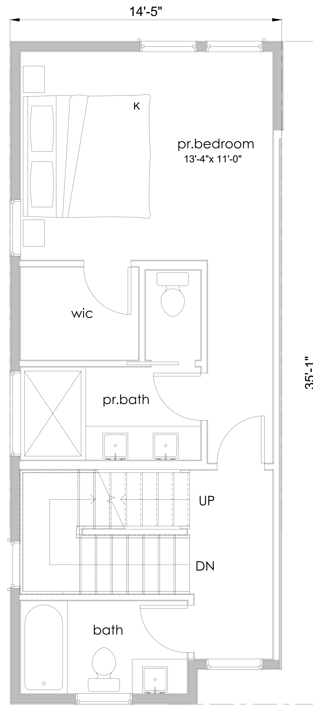
THIRD FLOOR
