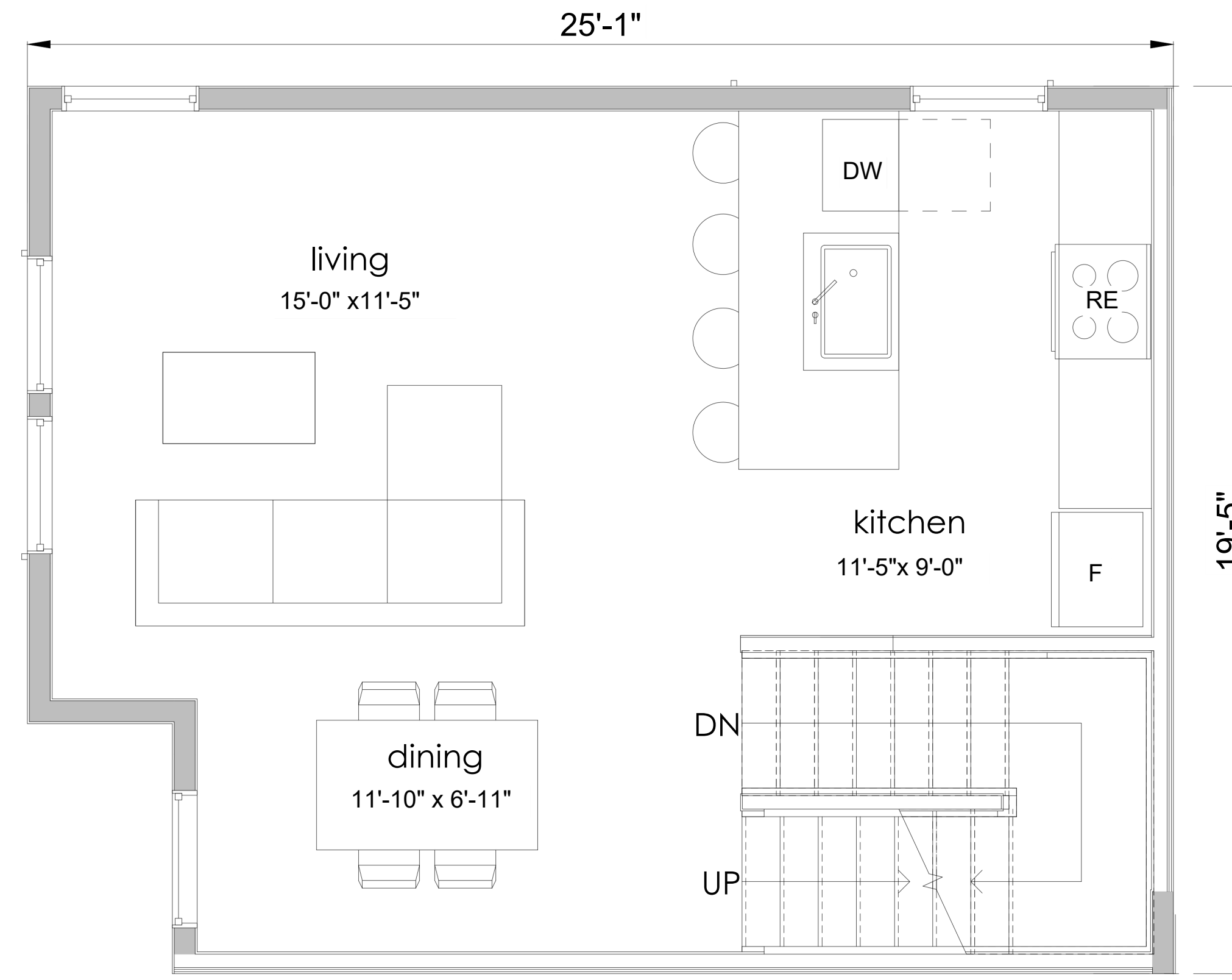
SECOND FLOOR
