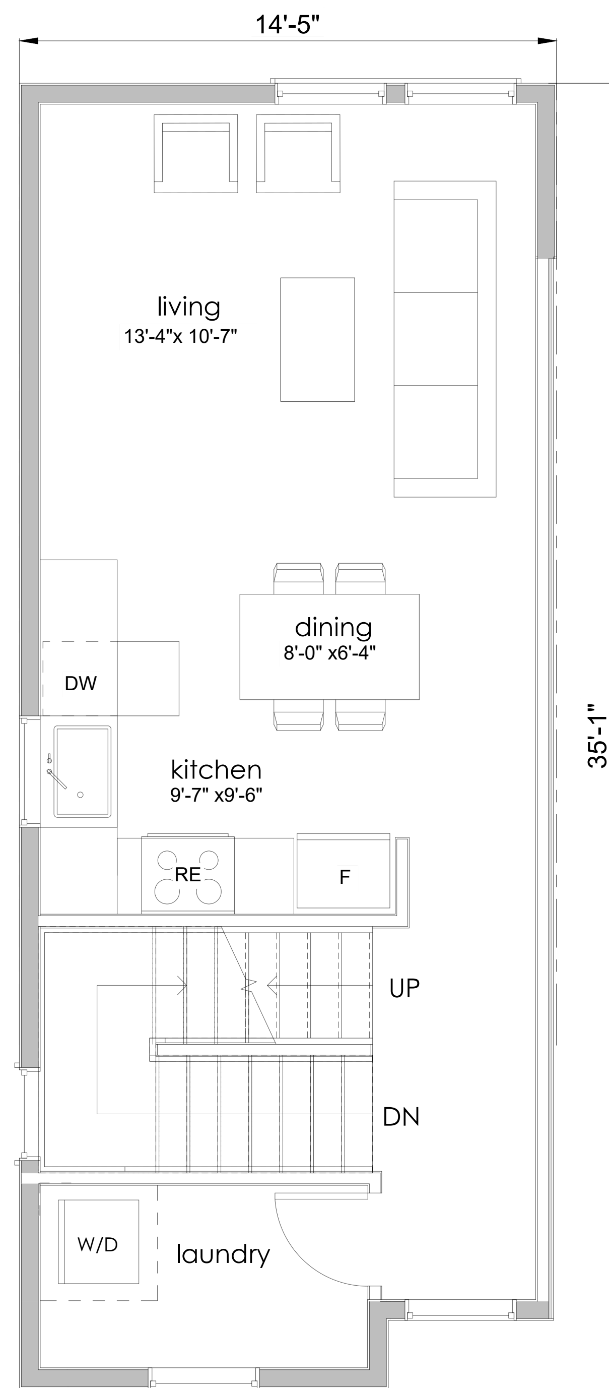
SECOND FLOOR
