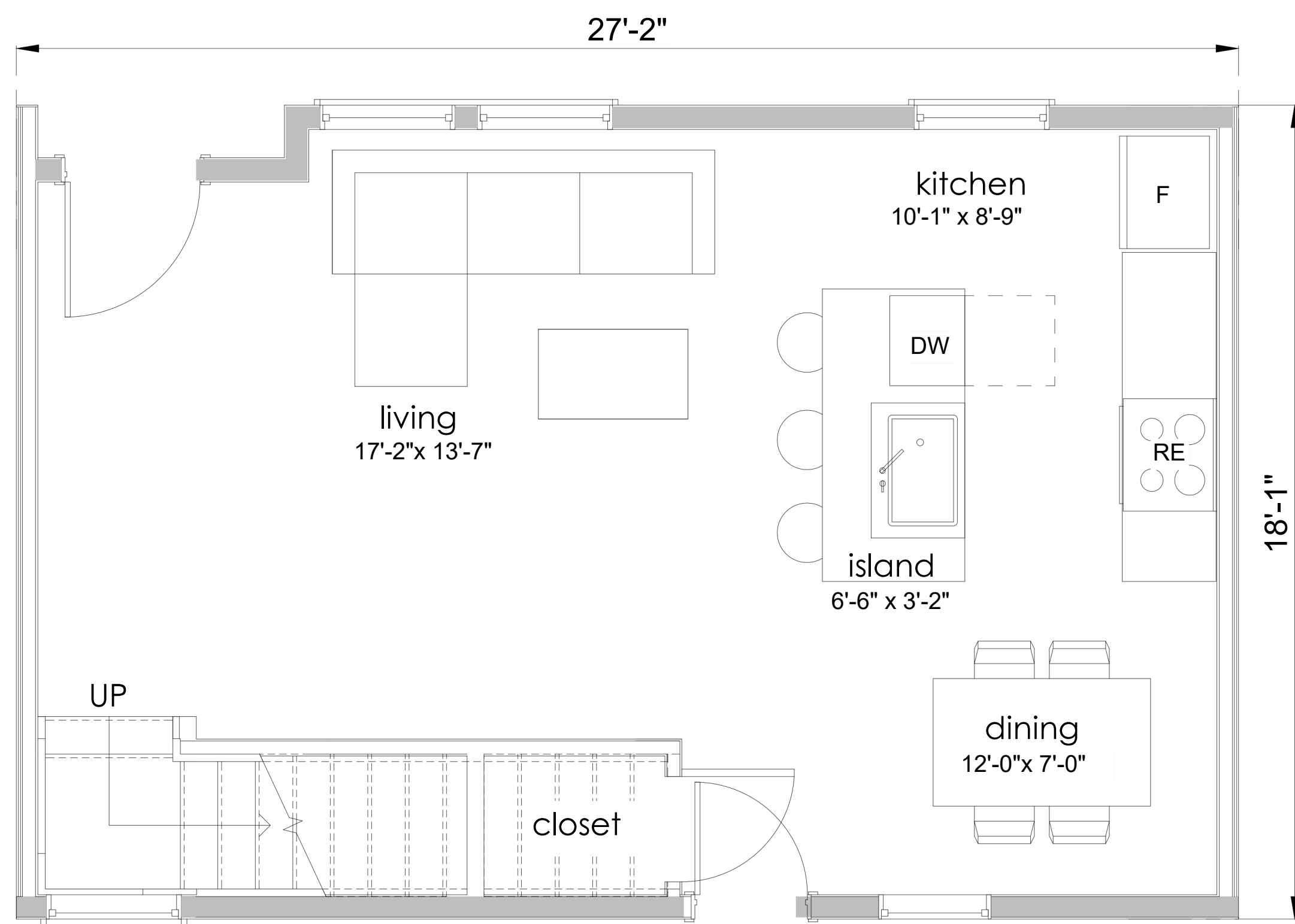
FIRST FLOOR
